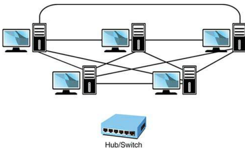
FIGURE 1.4 Mesh topology
