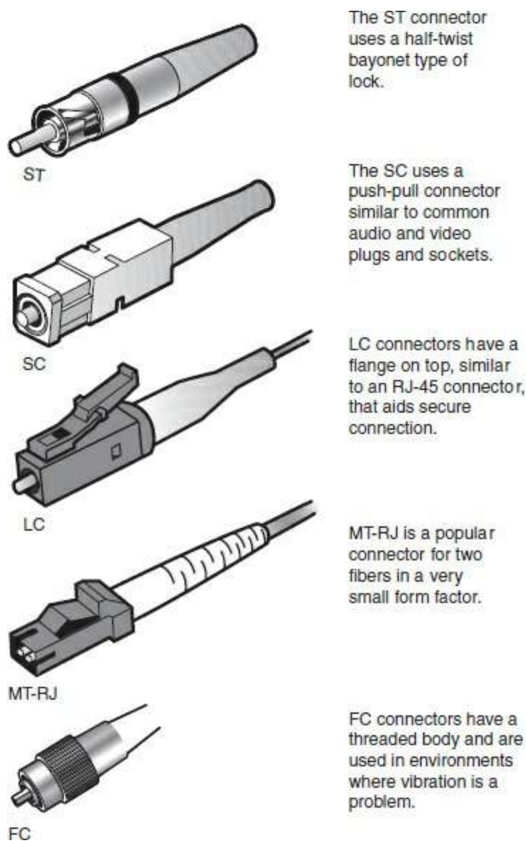
FIGURE 6.8 Fiber connectors
