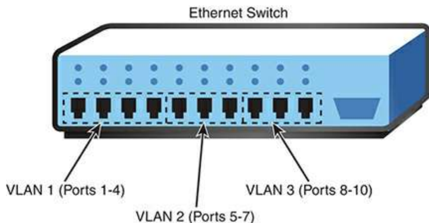
FIGURE 3.5 Port-based VLAN membership
