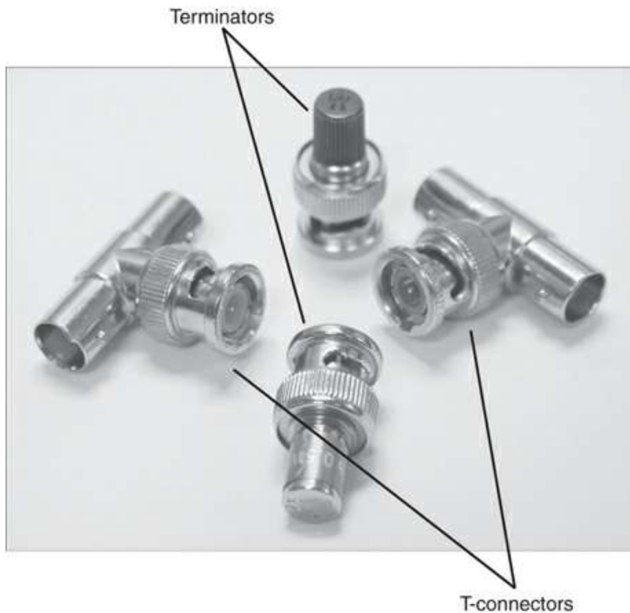
FIGURE 6.4 BNC connectors
