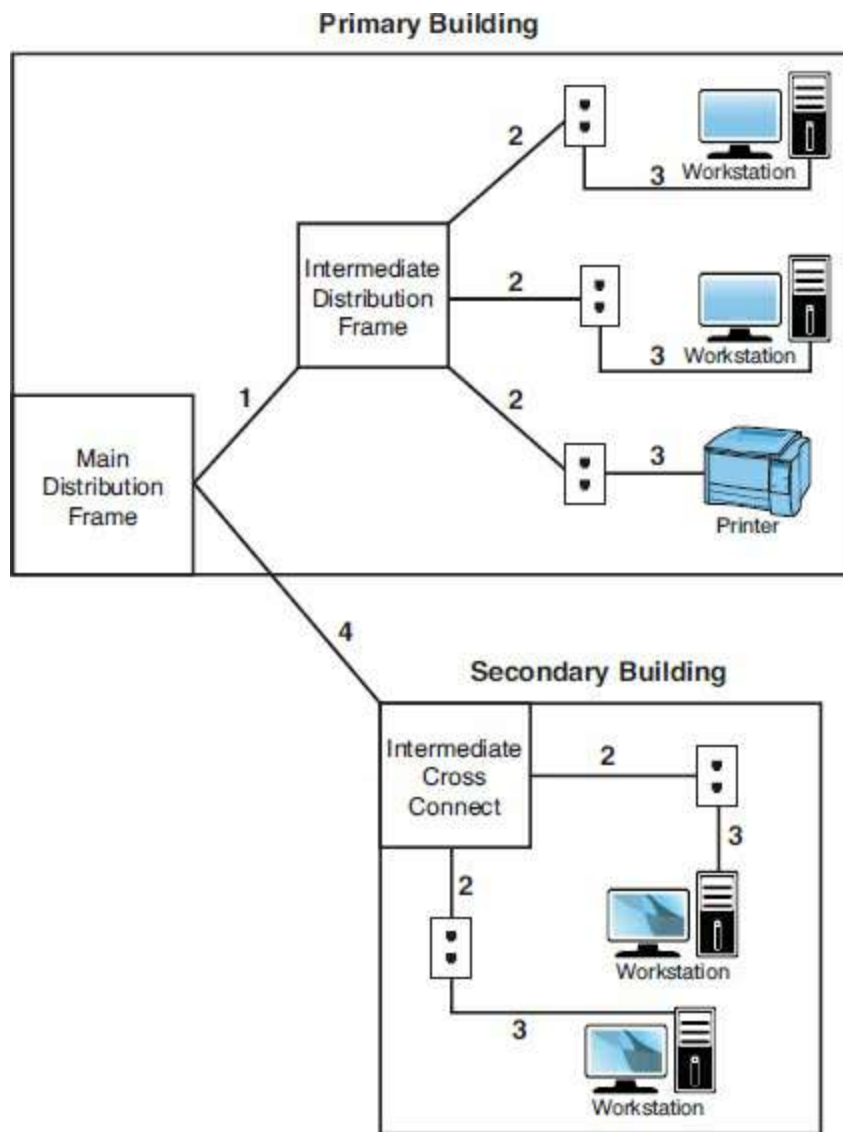
FIGURE 9.2 A general wiring schematic
