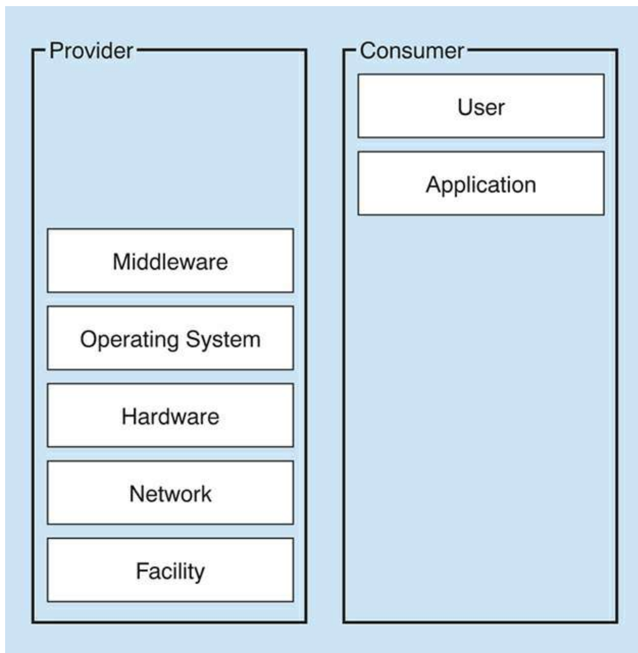
FIGURE 8.2 The PaaS service model
